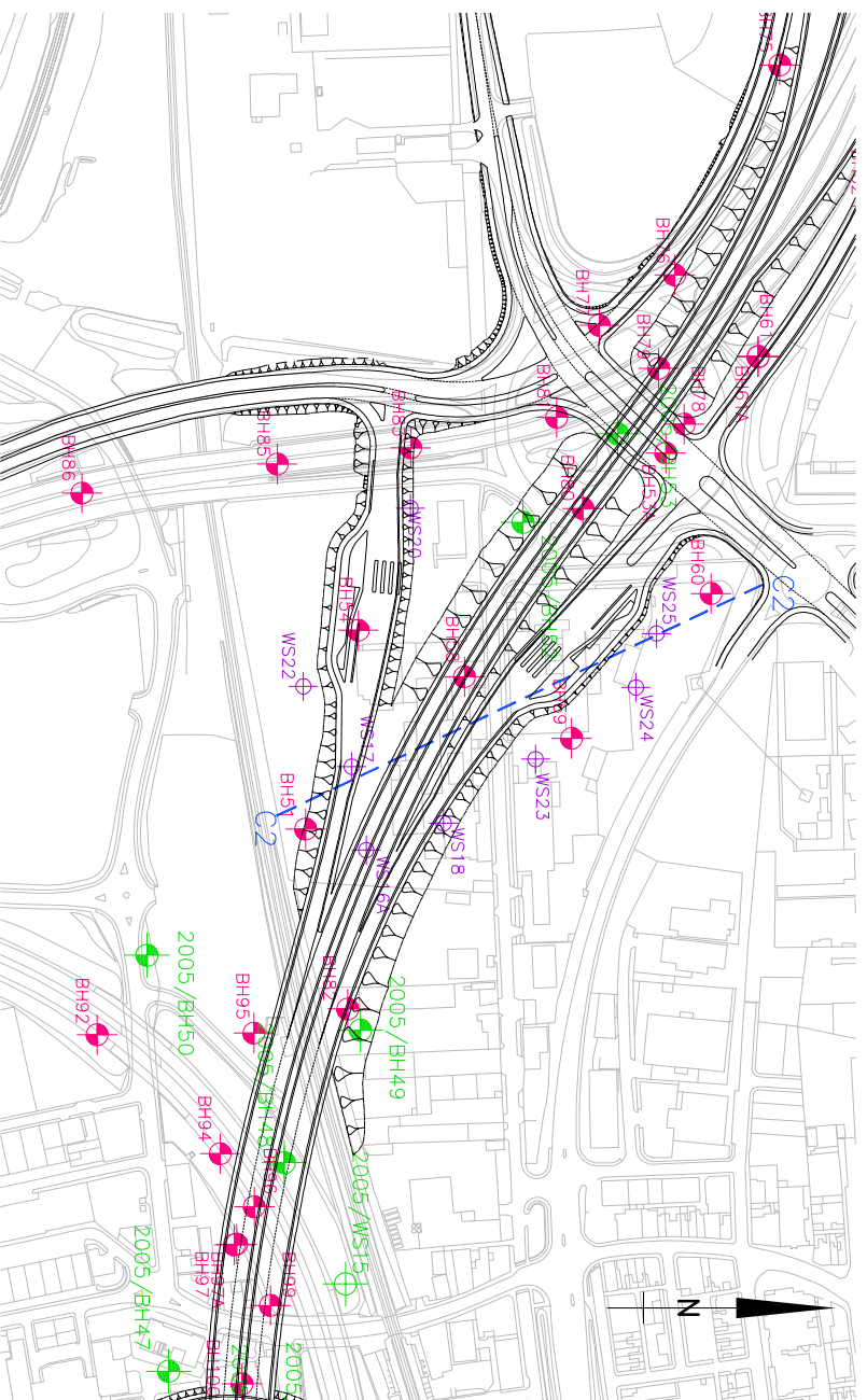
Plan view Section C2-C2 1:5000
